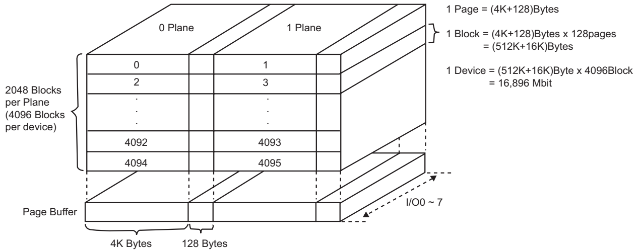
Figure 4: Array Organization
