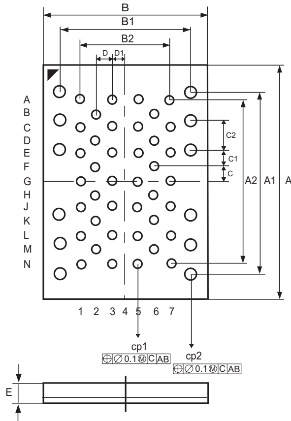
Figure 38: 52-VLGA, 14 x 18mm, Package Outline (Top view through package)
