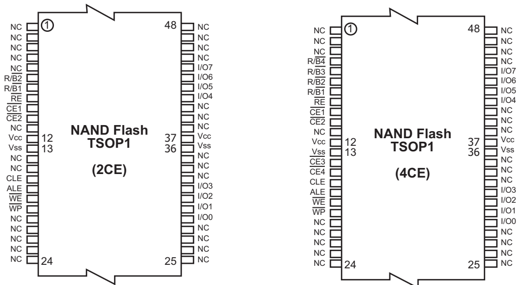
Figure 2: 48TSOP1 Contact, x8 Device
