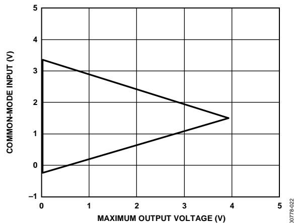
Figure 22. Maximum Output Voltage vs. Common-Mode Input, G = 1 , +V_S = 5 V , -V_S = 0 V , R_L = 100 k\Omega
