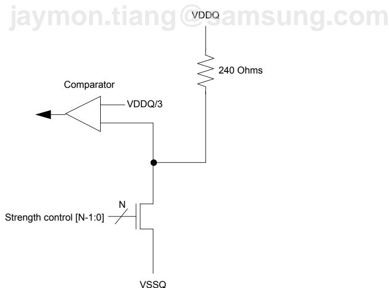
Figure 21. pull-down calibration
